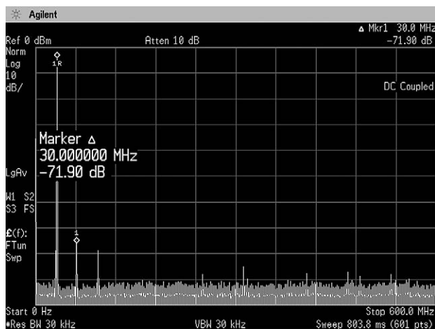
Figure 10. Spurious performance outstanding at low signal frequencies.
